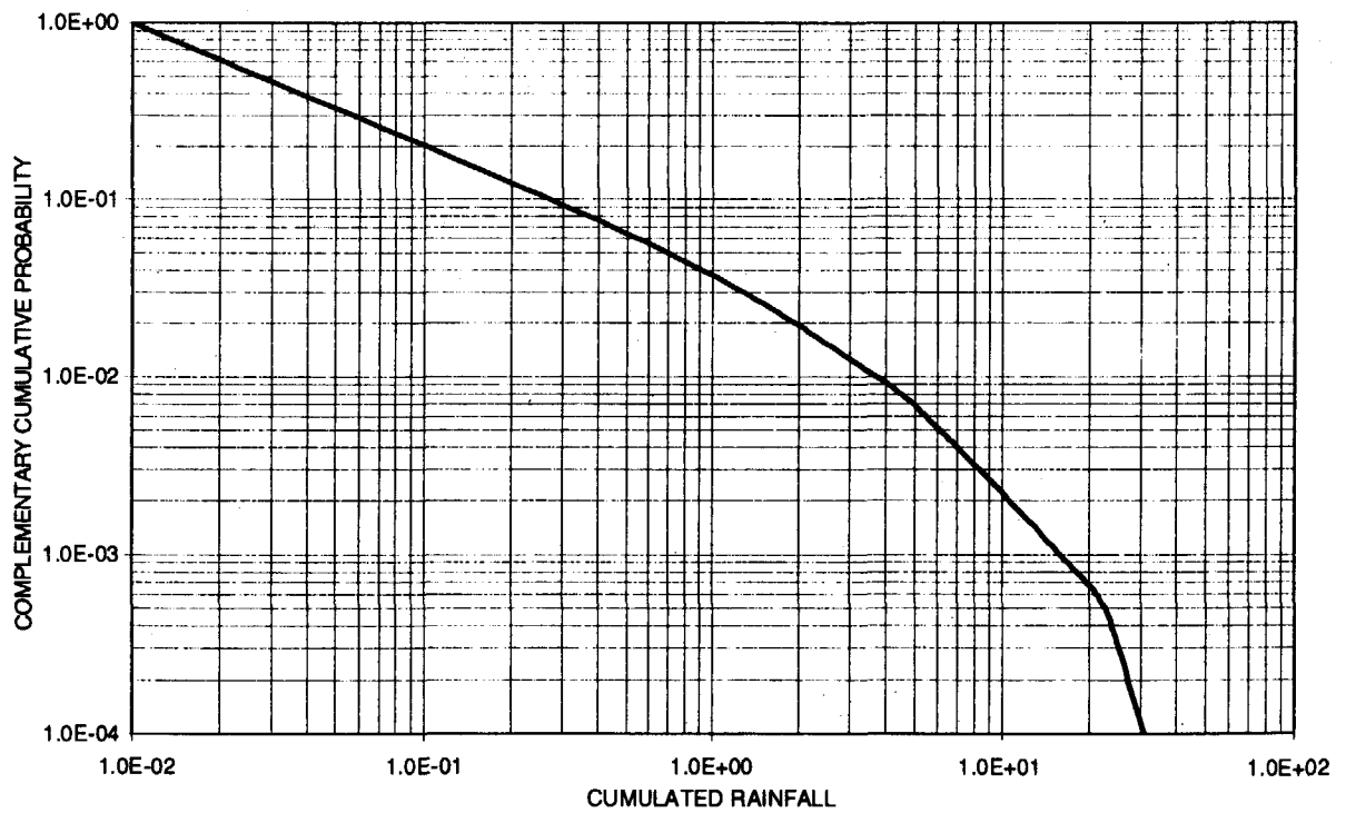
Figure 10. Probabilistic distribution of cumulated rainfall within 10km
